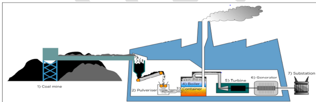
The process of making electricity from coal in a power station
